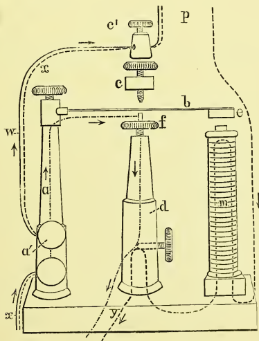
FIG. 6. THE MAGNETIC INTERRUPTER WITH HELMHOLTZ ARRANGEMENT FOR EQUALIZING THE MAKE AND BREAK SHOCKS.
